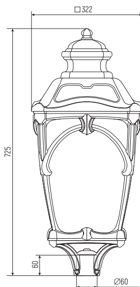
Post Top
